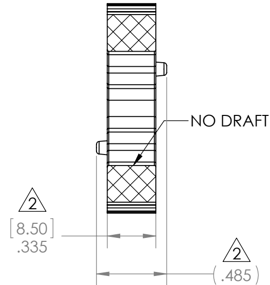
SECTION C-C
